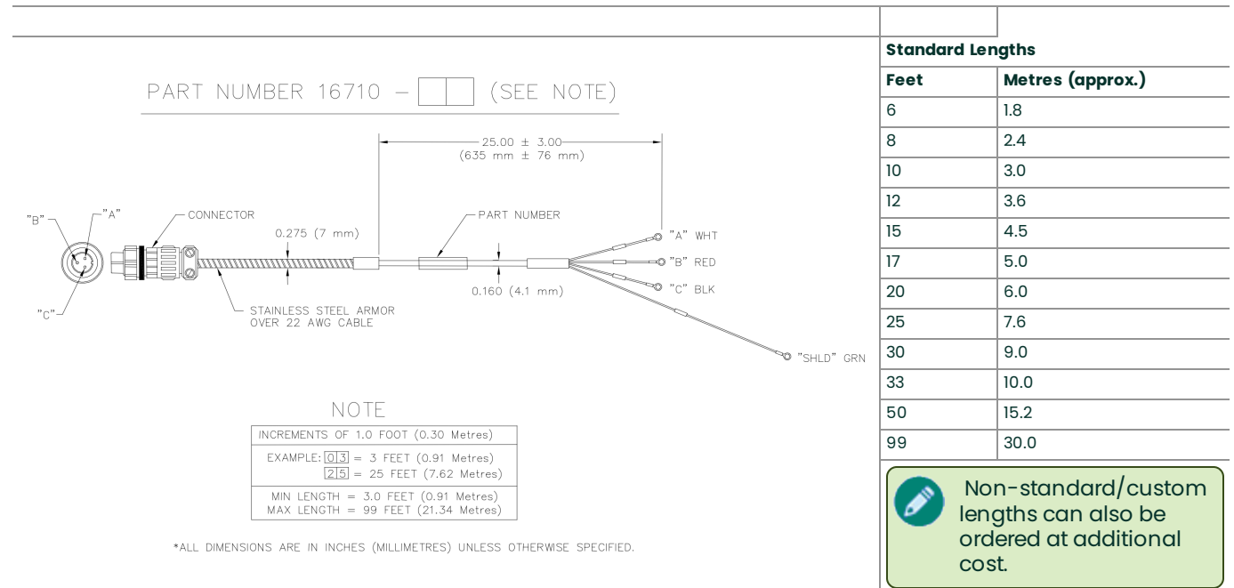
Figure 4: Standard Interconnect Cable
